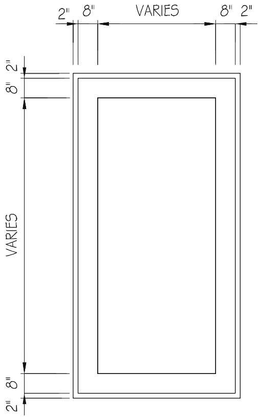
WALL PLAN VIEW
